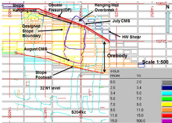
Figure 3. Block 1 32s 204 stope; 32N1 level plan.
