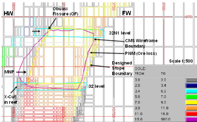
Figure 4. Cross section along A – A1 of block 1 32s 204 stope (looking North).
