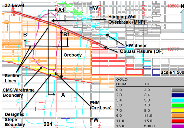
Figure 2. Block 1 32s 204 Stope; 32 level plan showing section lines (A – A1 and B – B1).
