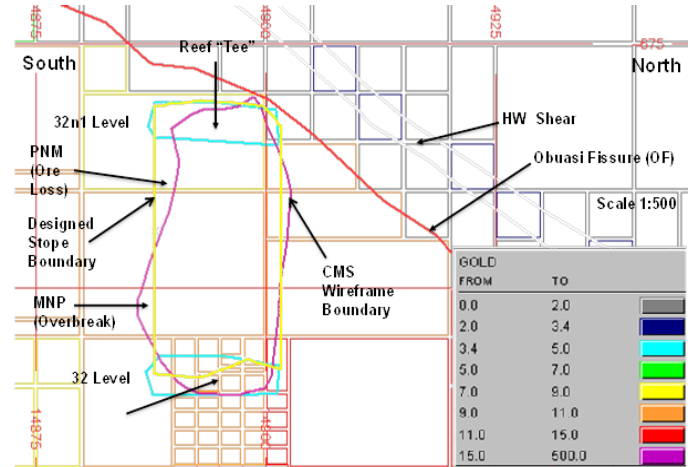
Figure 5. Longitudinal Section along B – B1 of Block 1 32s 204 Stope, showing lateral Overbreak and Underbreak.
