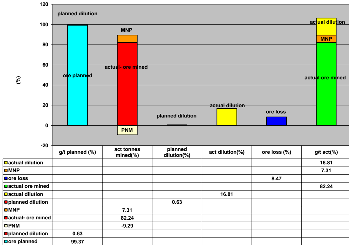
Figure 6. 32s 204 Stope performance graph.
